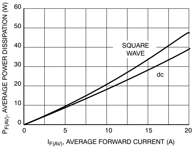
Figure 4. Power Dissipation
